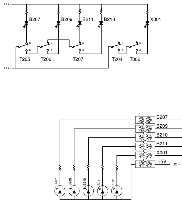
LED Schematic
