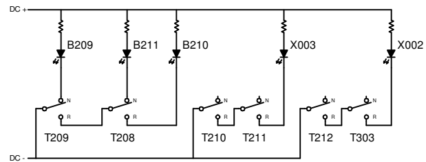
LED Schematic
